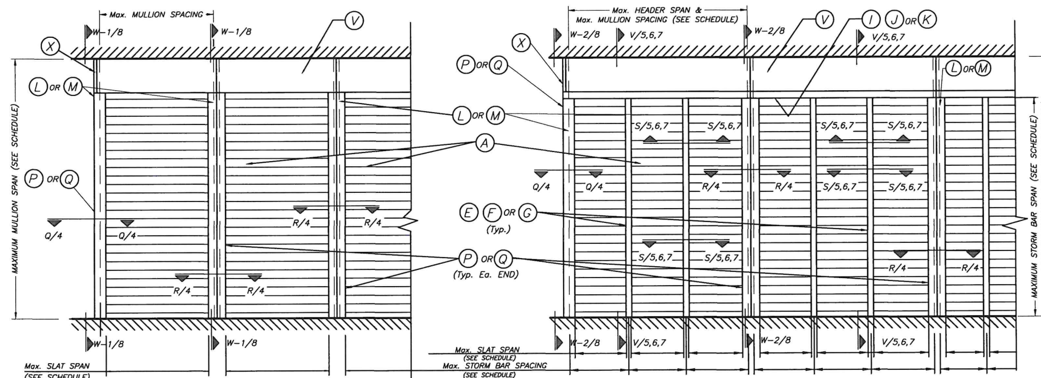
TYPICAL CONSECUTIVE SINGLE UNIT ELEVATION (NO STORM BARS REQUIRED) NOTE: SEE SHEET 2 & 3 OF 11 FOR COMPONENTS NOMENCLATURE. TYPICAL CONSECUTIVE MULTIPLE UNIT ELEVATION (STORM BARS REQUIRED) NOTE: SEE SHEET 2 & 3 OF 11 FOR COMPONENTS NOMENCLATURE.
