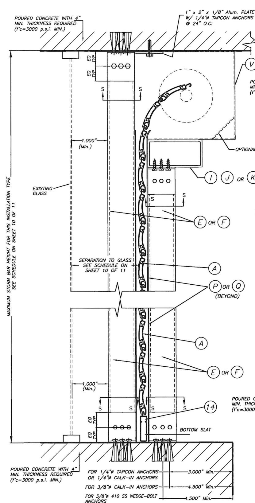
CEILING & FLOOR MOUNTING: SECTION V-V(2) INSTALLATION W/ FIXED OR REMOVABLE STORM BARS W/CONCRETE ANCHORS (SEE SECTION "S" FOR ANCHOR TYPE REQUIREMENT) SCALE : N.T.S.
