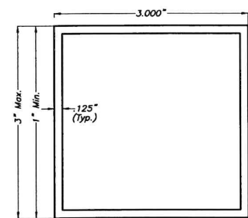
Y BUILD-OUT TUBES 3"x3" EXTRUDED TUBE 6063-T5 ALUMINUM ALLOY
