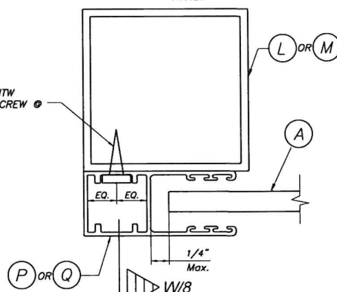
SECTION Q - Q : MULLION MOUNT N.T.S.
