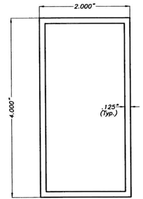
F TYPE 2 STORM BAR: 4" EXTRUDED STORM BARS 6063-T6 ALUMINUM ALLOY
