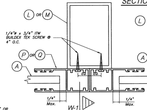
SECTION R - R : MULLION MOUNT N.T.S.
