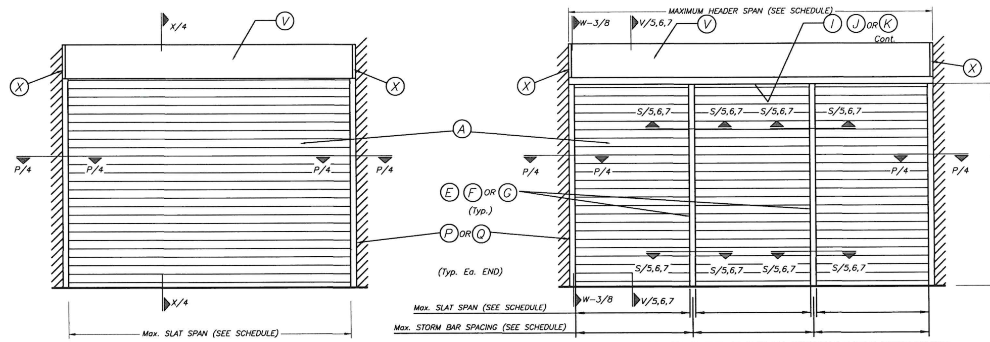
TYPICAL SINGLE UNIT ELEVATION (NO STORM BARS REQUIRED) NOTE: SEE SHEET 2 & 3 OF 11 FOR COMPONENTS NOMENCLATURE. TYPICAL MULTIPLE UNIT ELEVATION (STORM BARS REQUIRED) NOTE: SEE SHEET 2 & 3 OF 11 FOR COMPONENTS NOMENCLATURE.
