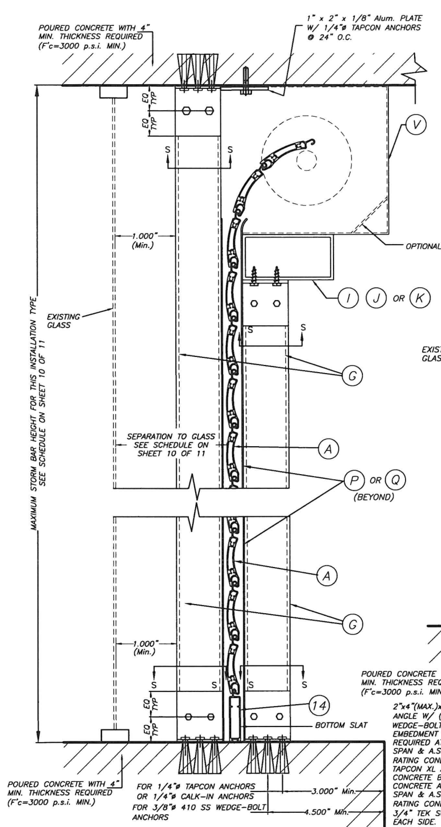
CEILING & FLOOR MOUNTING: SECTION V-V(2) INSTALLATION W/ FIXED OR REMOVABLE STORM BARS W/CONCRETE ANCHORS (SEE SECTION "S" FOR ANCHOR TYPE REQUIREMENT)
