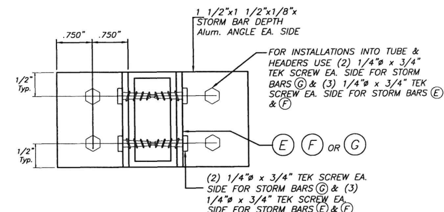
SECTION S3 - S3 SCALE : 1/2" = 1"
